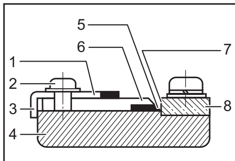
► 1. Adjust plate 2. Screws 3. Heel of adjust plate 4. Back side of gauge base 5. Blade edge 6. Planer blade 7. Inside edge of gauge plate 8. Gauge plate
