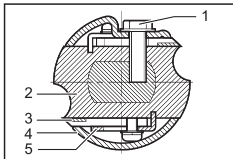
► 1. Bolt 2. Drum 3. Planer blade 4. Drum cover 5. Adjust plate
